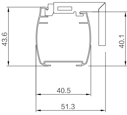
Bead Chain/ Motorized Headrail Screw Fix
