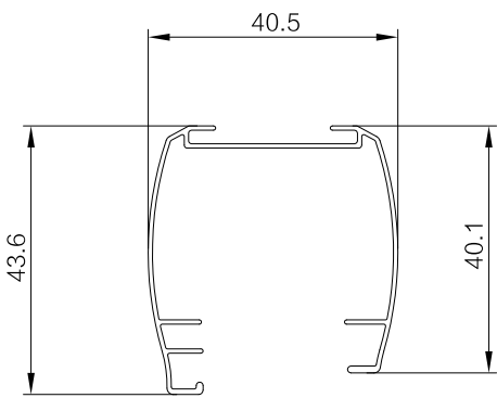
Bead Chain/ Motorized Headrail No Drill Blinds
